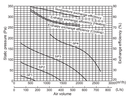
LGH-250RVXT-E
