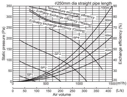
LGH-150RVXT-E
