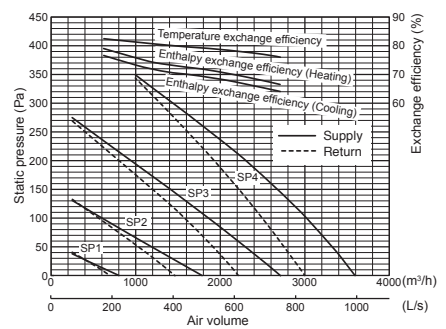
GUF-100RDH4
