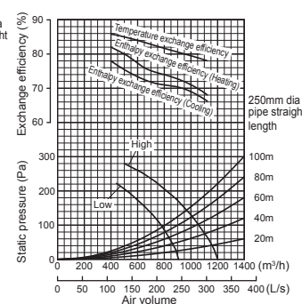
GUF-100RDH4
