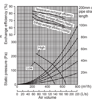
GUF-50RDH4
